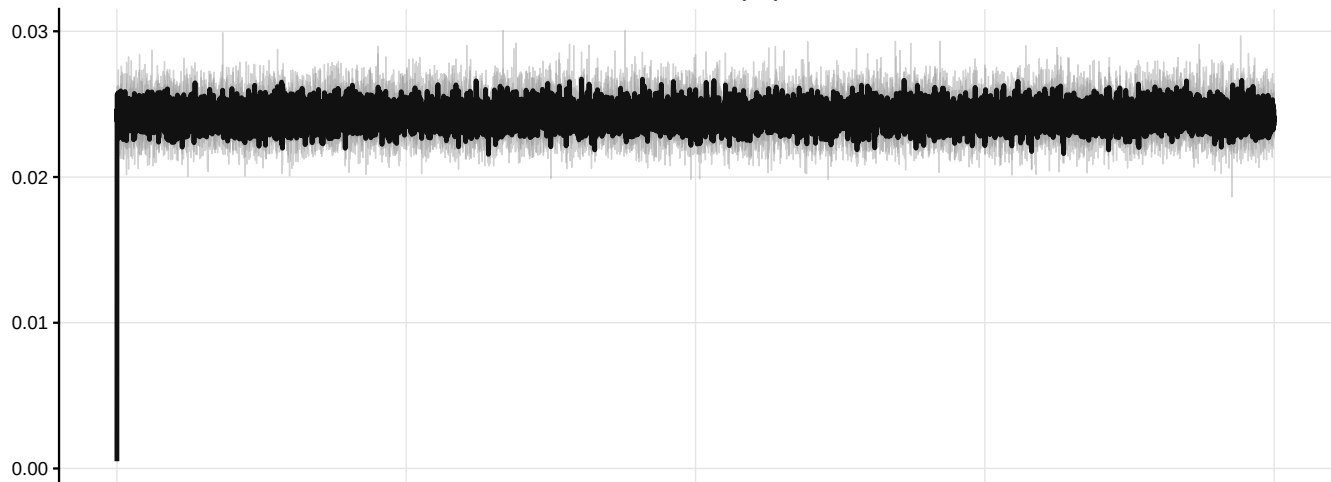
Radius of gyration (nm)
