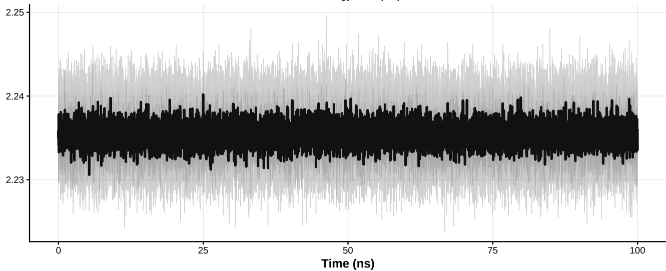
Radius of gyration (nm)
