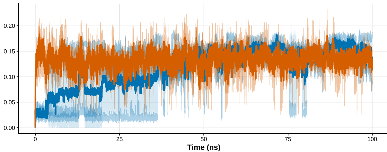
Self RMSD
