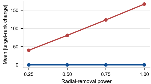
Target-rank displacement
