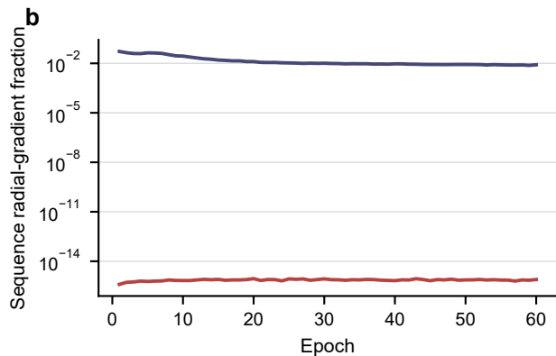
Beauty mechanism trace (seed 2025; identical architecture and optimiser)
