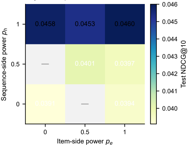
a Beauty fixed- \tau partial-normalisation screen
