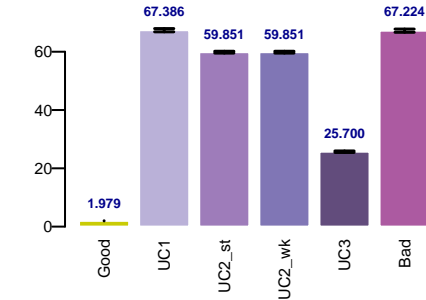
percent_see
