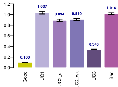
rmse
