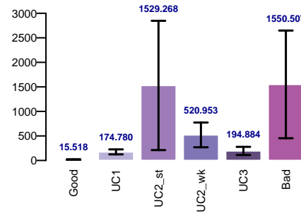
percent_see
