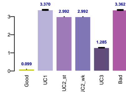
median_ae
