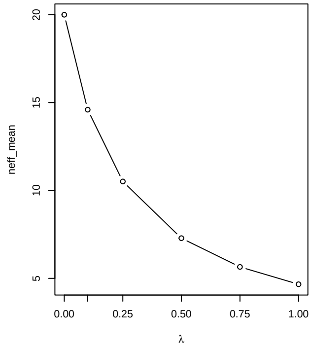
Effective sample size
