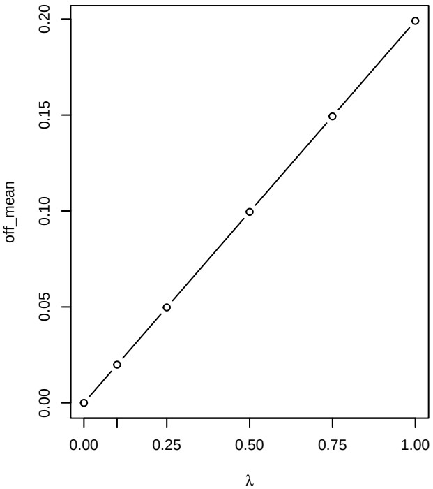
Mean off-diagonal correlation
