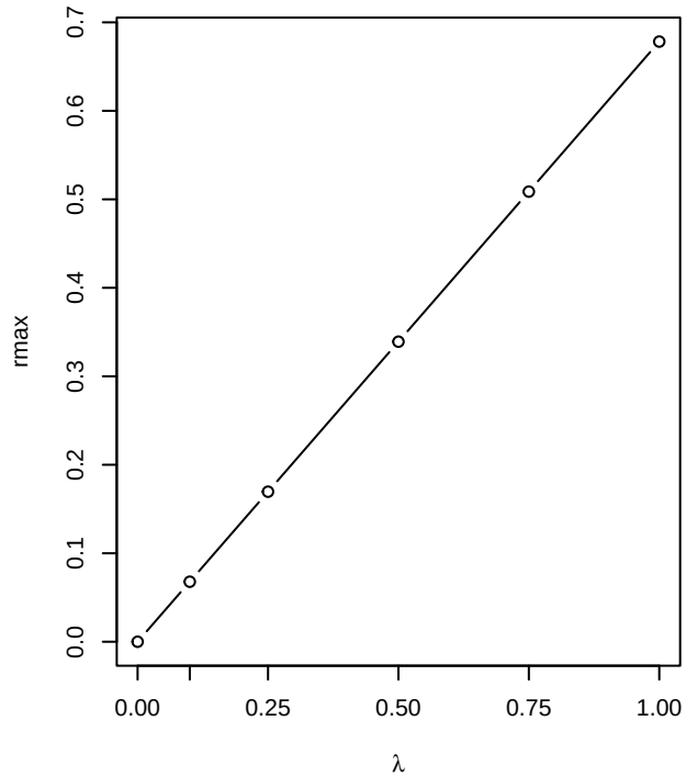
Maximum off-diagonal correlation
