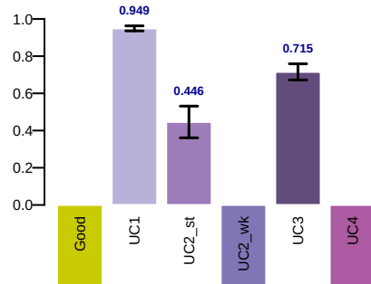
whitened_r2
