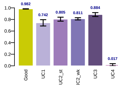
pic_spearman
