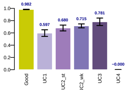
pic_r2
