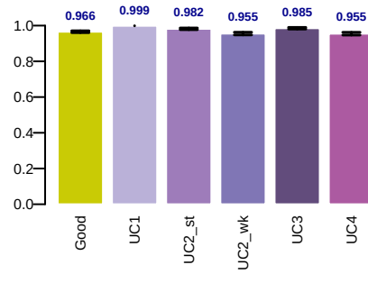
lik_r2
