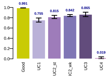
pic_pearson
