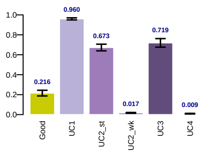
resid_r2
