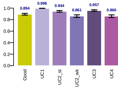
resid_r2
