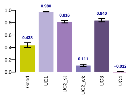
lik_r2
