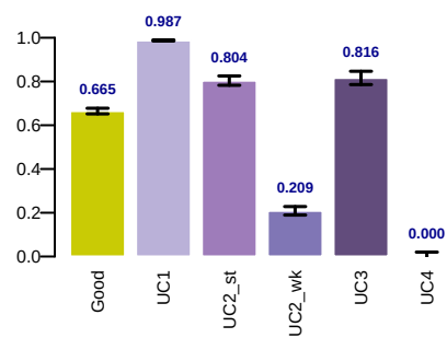
pic_spearman
