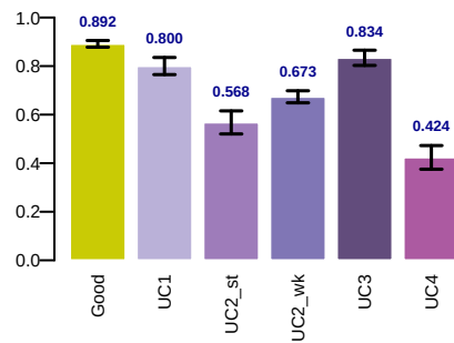
whitened_r2
