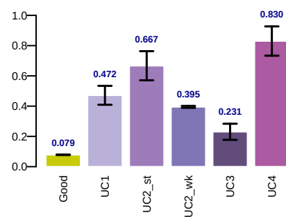
pic_rmse
