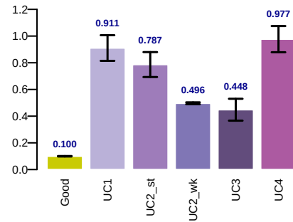
see
