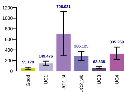
whitened_rmse
