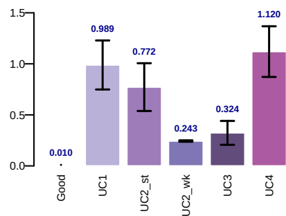
median_ae
