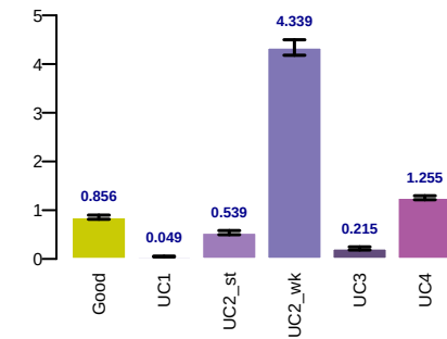
whitened_mae
