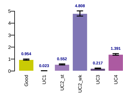
percent_see
