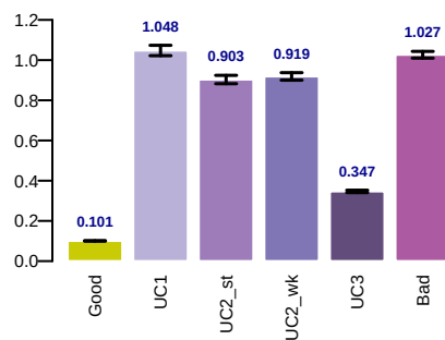
see
