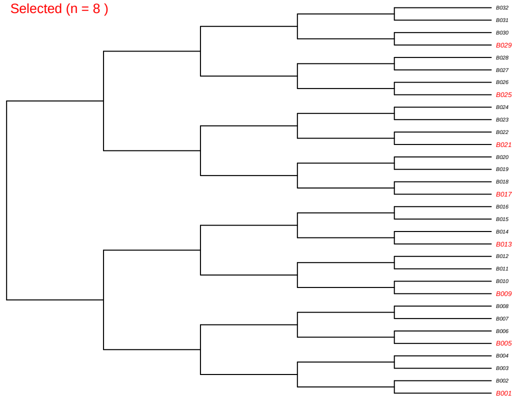
Balanced – Dispersed MeanESS = 4.44
