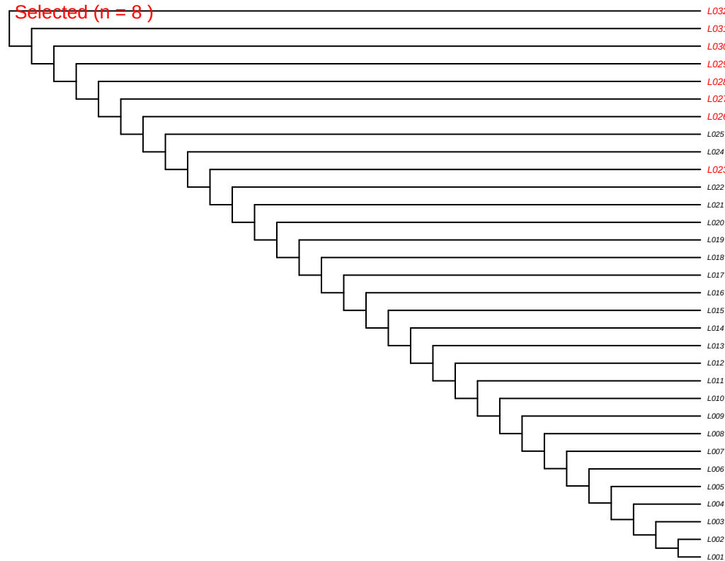
Ladder – Dispersed MeanESS = 5.70
