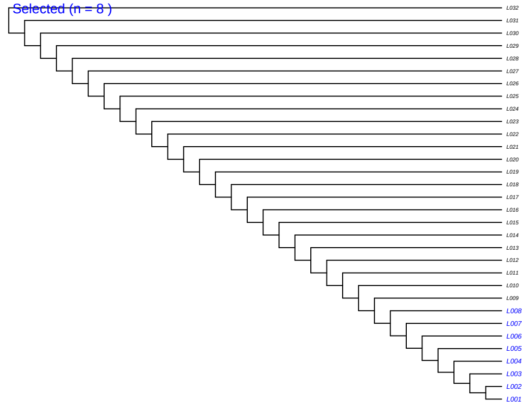
Ladder – Clustered MeanESS = 1.19
