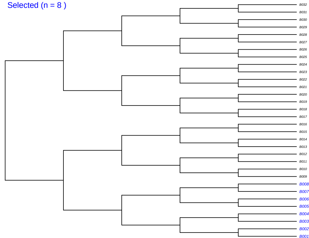
Balanced – Clustered MeanESS = 1.74
