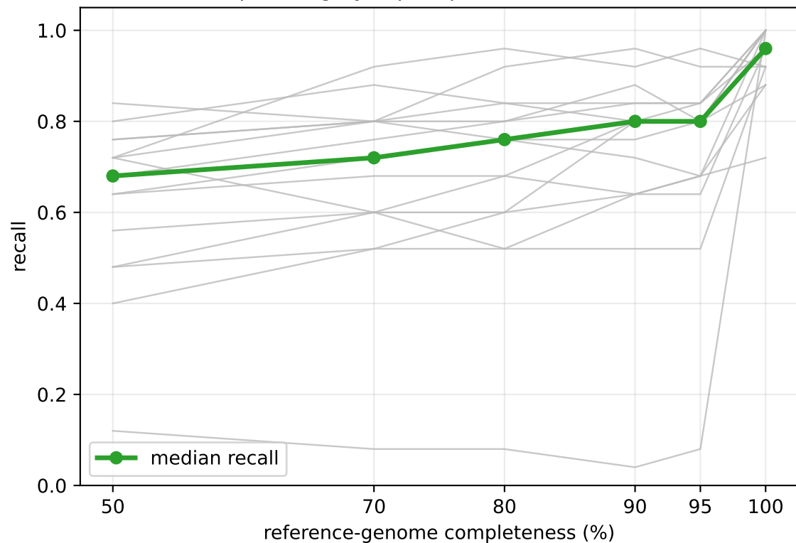
Recall vs reference completeness (15 species; grey = per species, bold = median)
