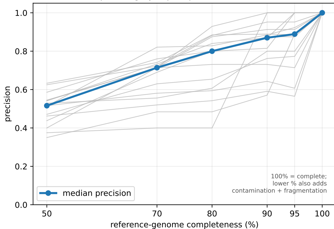
Precision vs reference completeness (15 species; grey = per species, bold = median)
