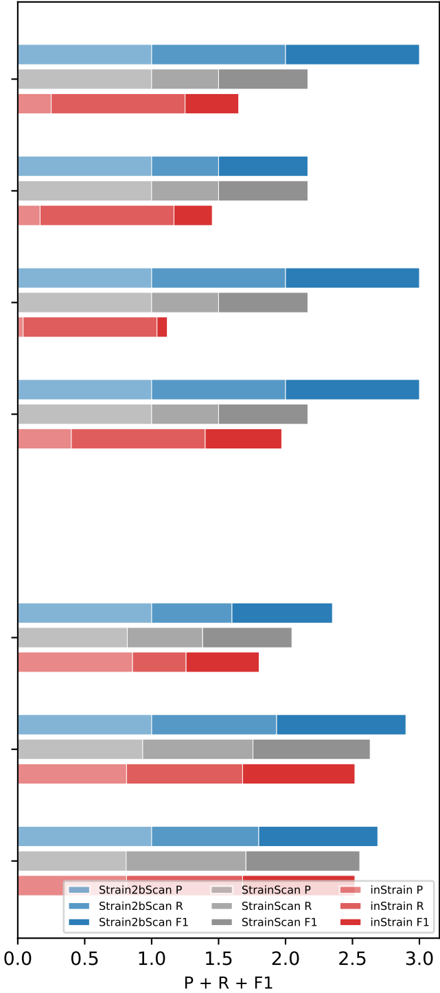
Performance
