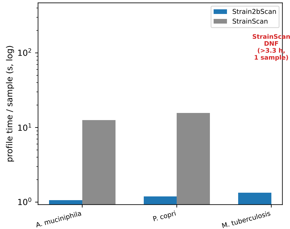
Profiling time per sample
