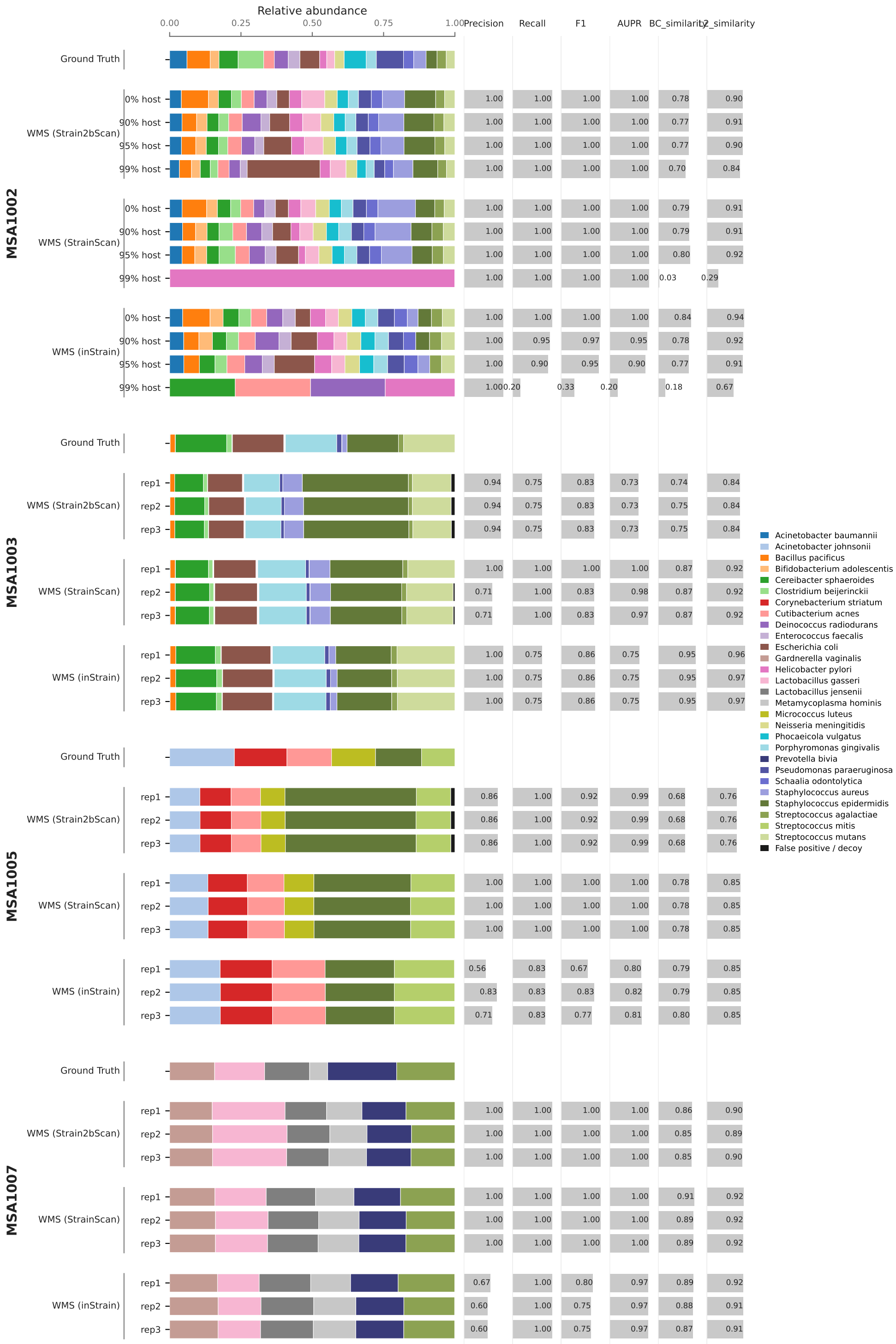
Figure 12 — Strain-level profiling on shotgun (WMS) mock communities
