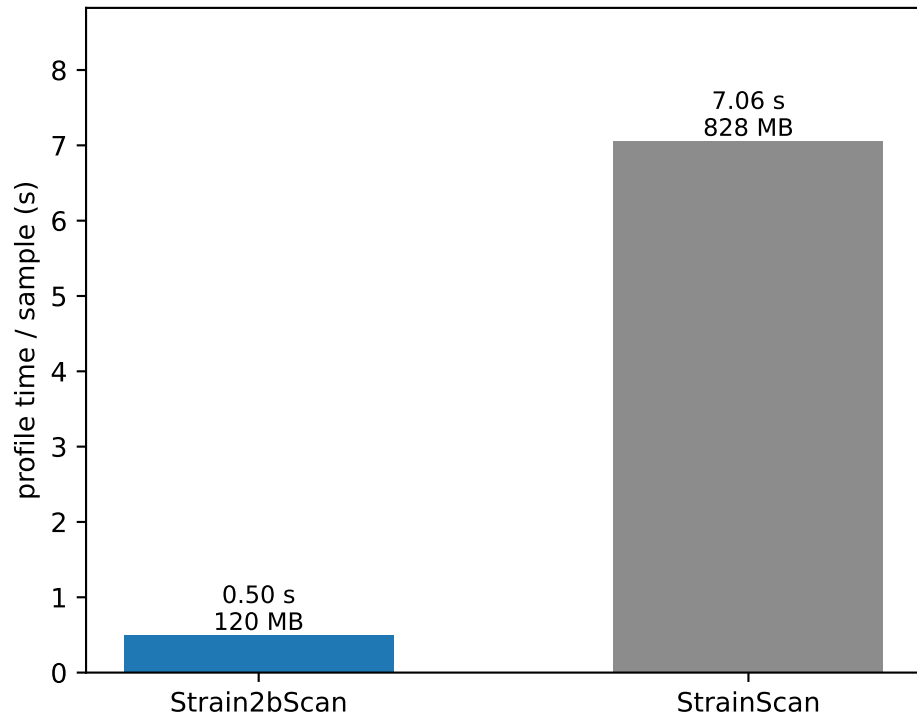
Per-sample profiling: \sim 14\times faster, \sim 7\times lighter
