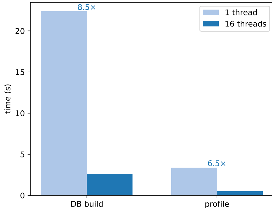
Parallel speedup (real C. acnes , 64 genomes)
