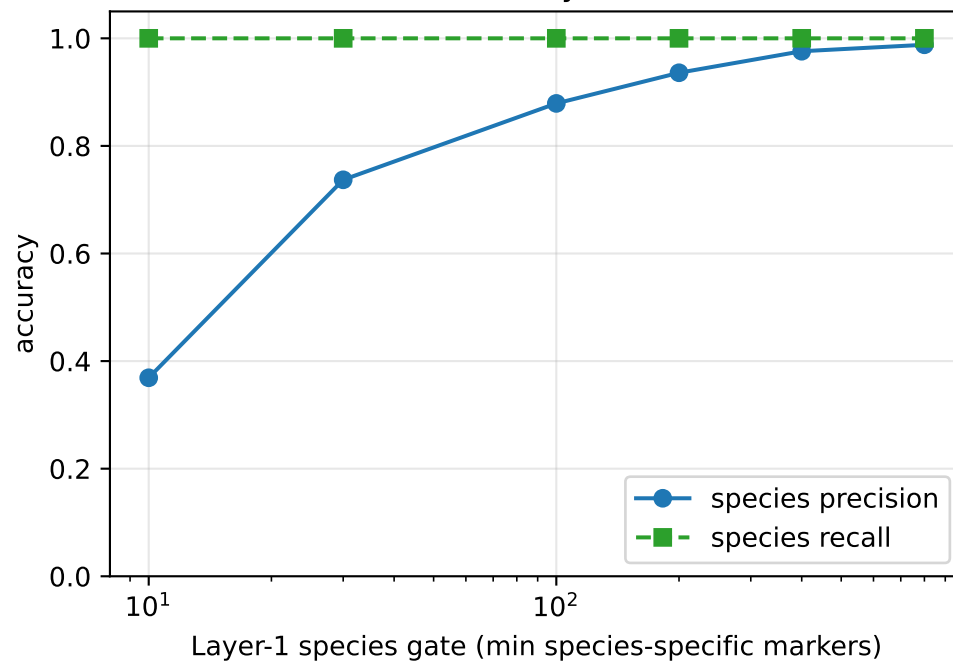
Multi-species accuracy vs species gate (recall stays 1.0)
