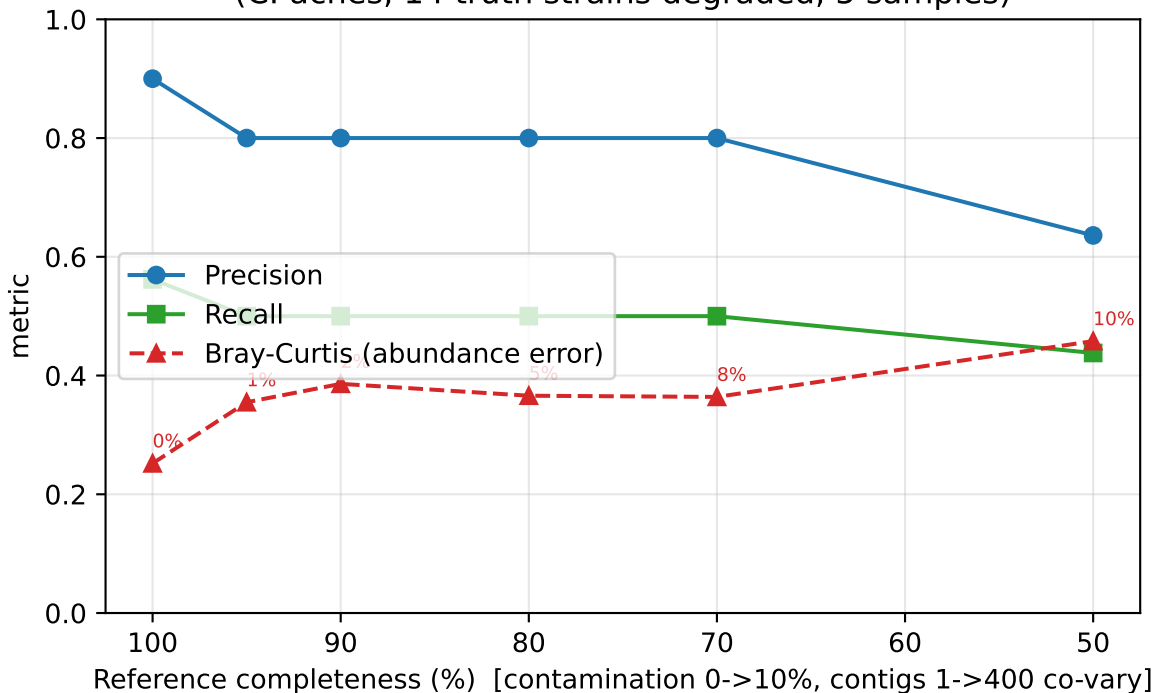
Reference-genome quality vs Strain2bScan accuracy ( C. acnes , 14 truth strains degraded, 5 samples)
