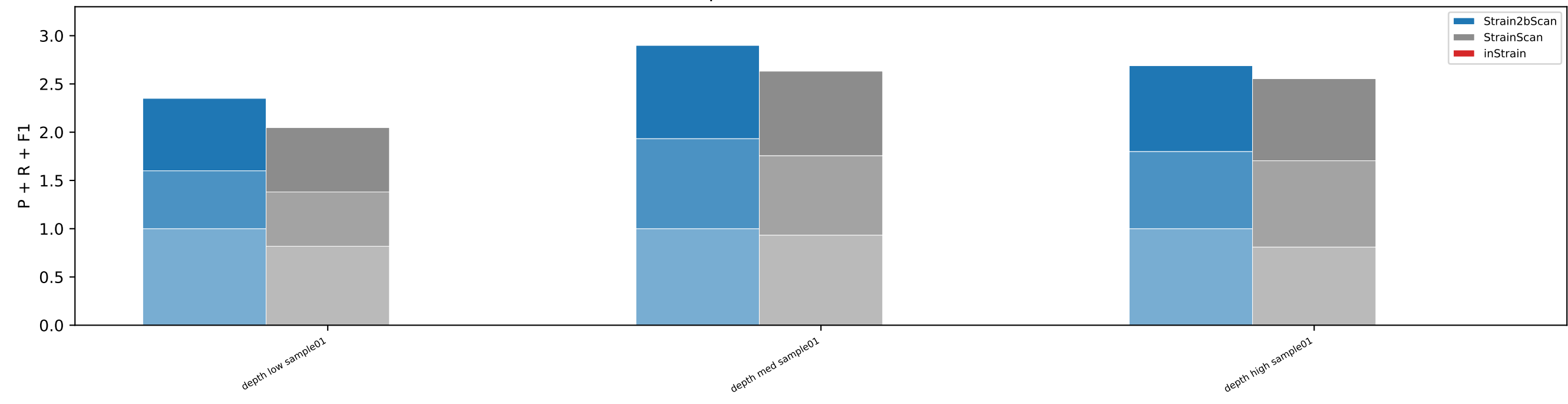
Multi-species simulated communities
