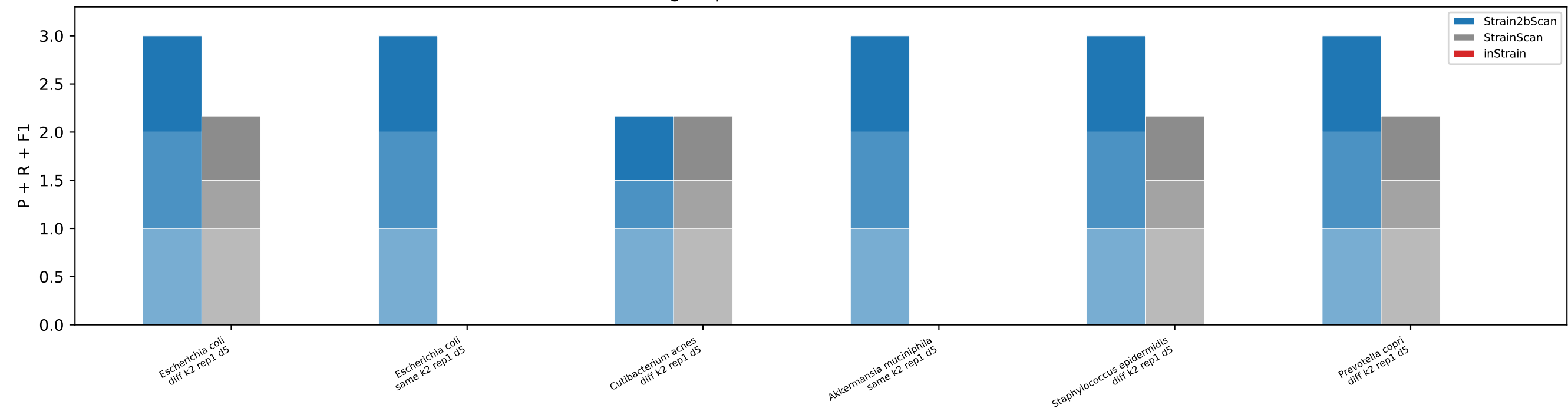
Single-species simulated communities
