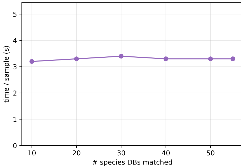
Species-count gradient — flat (digest once, match many; 10→55 species)
