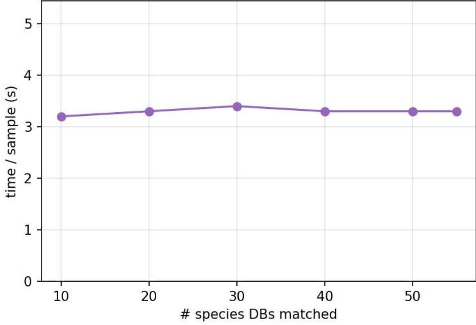
Species-count gradient — flat (digest once, match many; 10→55 species)
