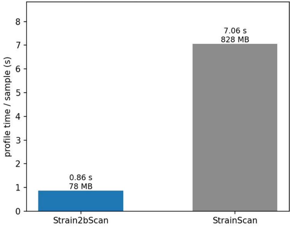
Per-sample profiling: ~8× faster, ~11× lighter
