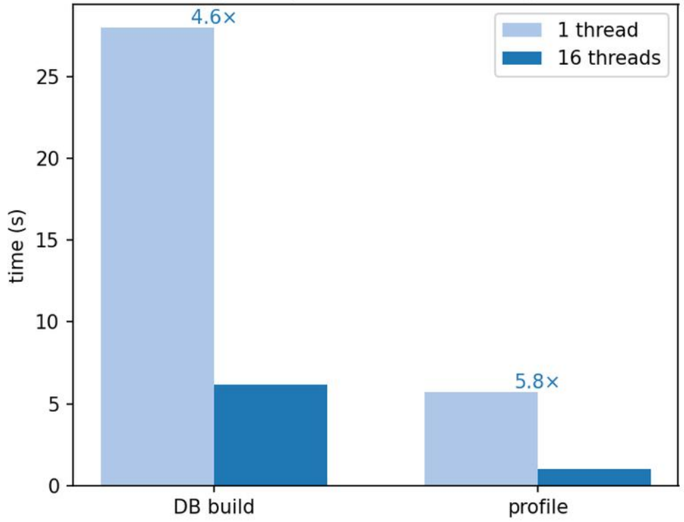
Parallel speedup (real C. acnes , 64 genomes)
