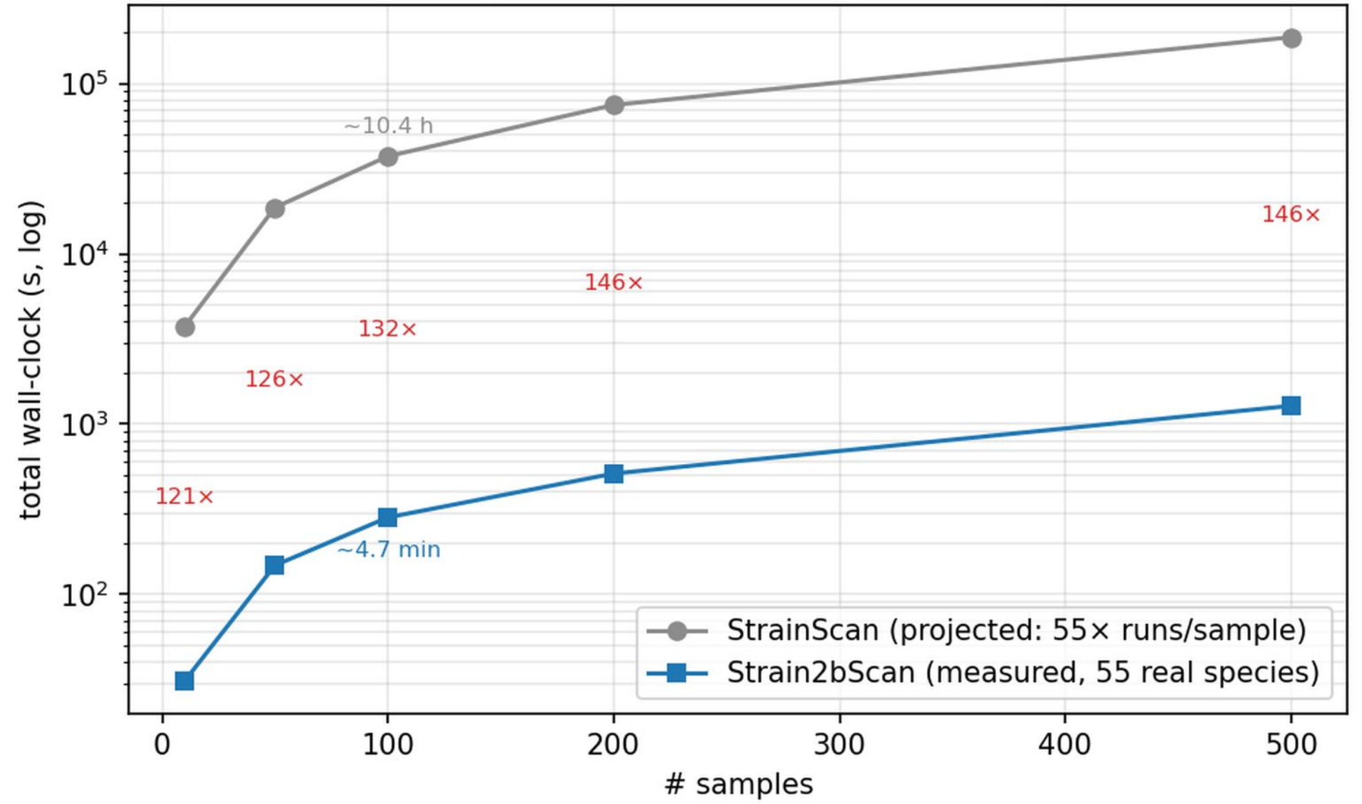
Community-scale strain profiling (55 real species)
