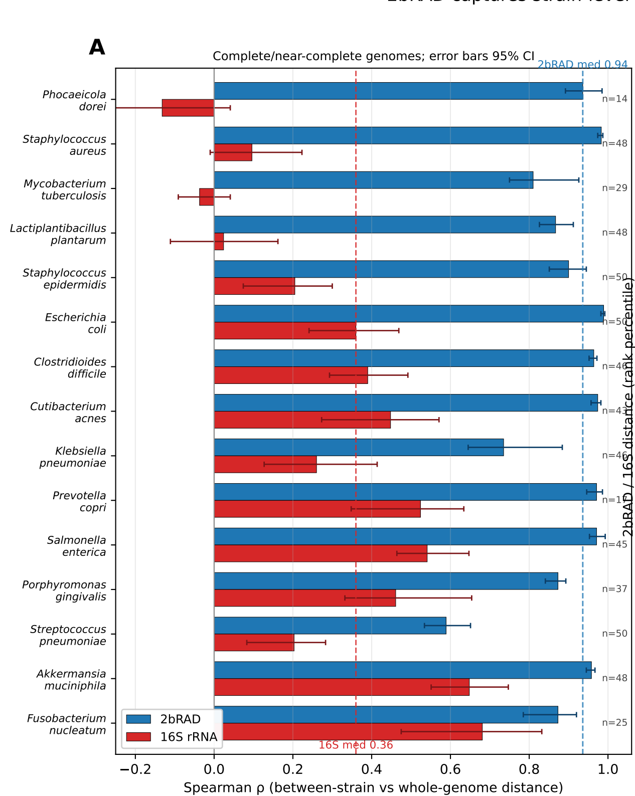
2bRAD captures strain-level signal that 16S cannot (15 species): summary (A) and per-species rank-rank scatter (B)
