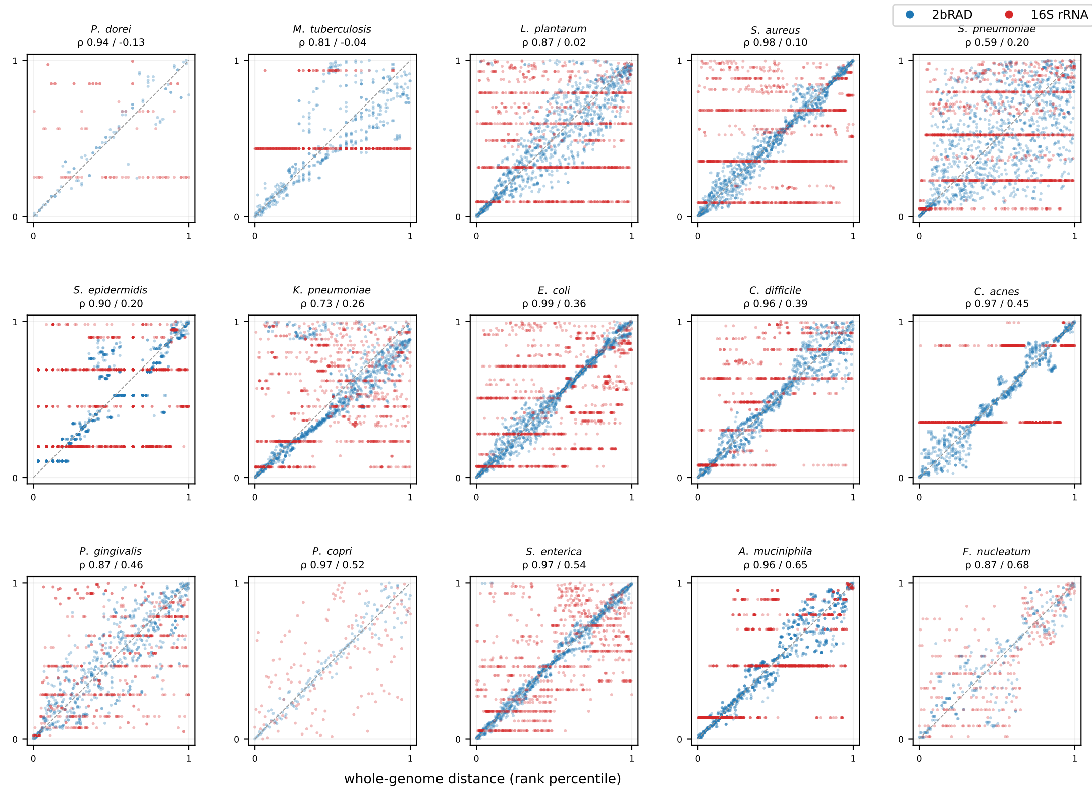
2bRAD captures strain-level signal that 16S cannot (15 species): summary (A) and per-species rank-rank scatter (B)
