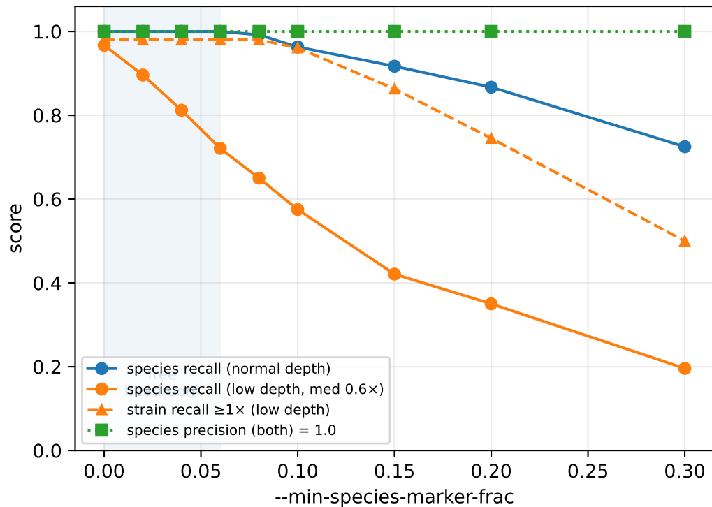
Floor=200: breadth term only trades recall (precision stays 1.0 at both depths)
