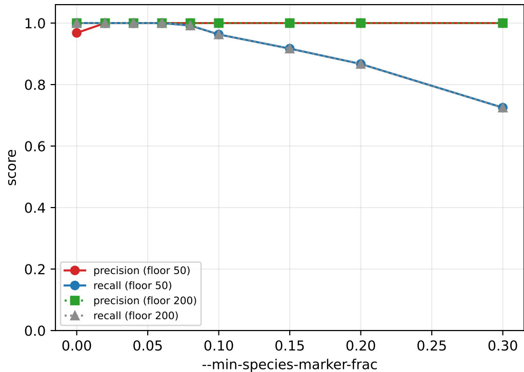
Relaxing the floor (200→50): where the breadth term earns its keep
