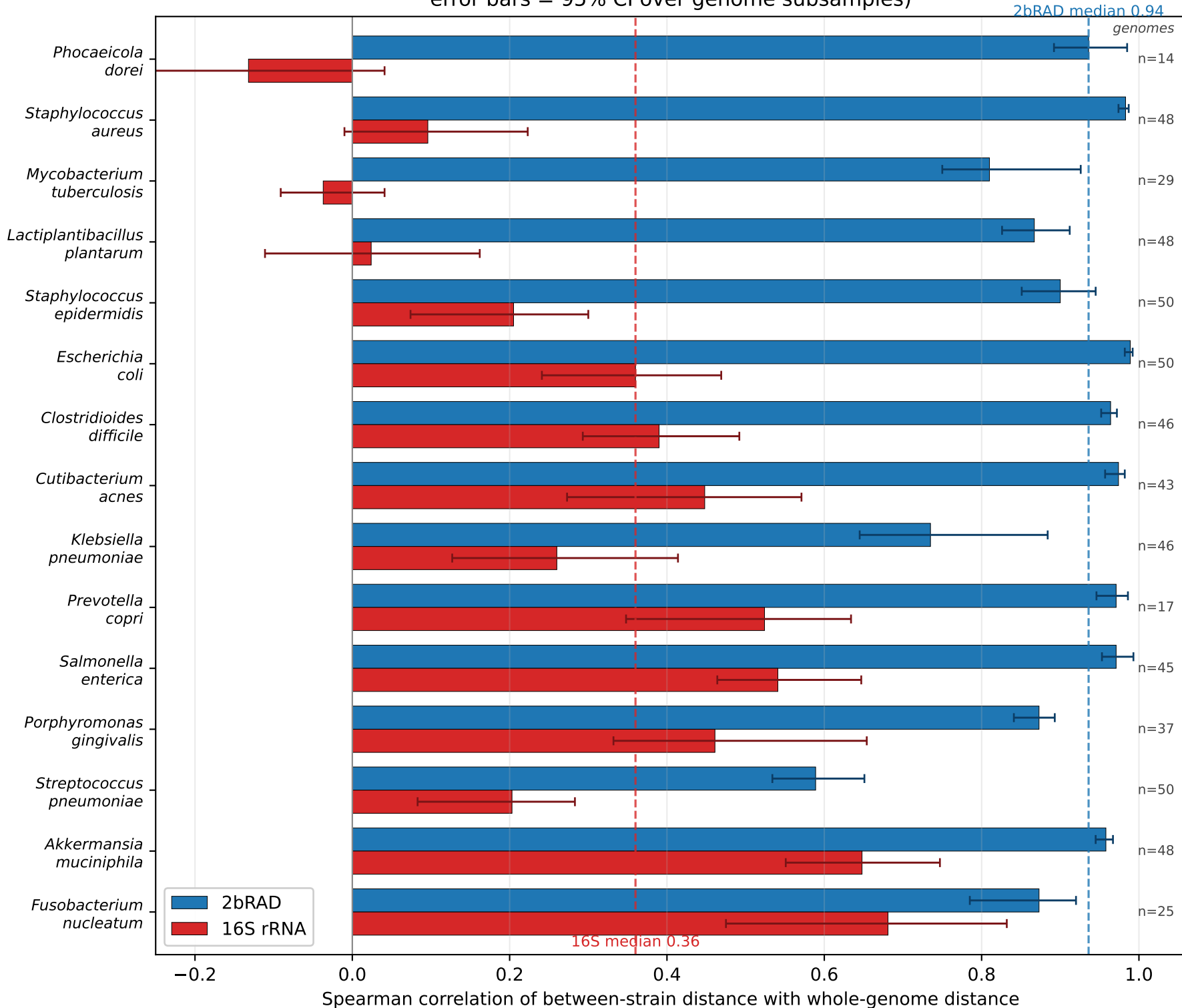
2bRAD captures strain-level signal that 16S cannot (between-strain vs whole-genome distance; complete/near-complete genomes; error bars = 95% CI over genome subsamples)
