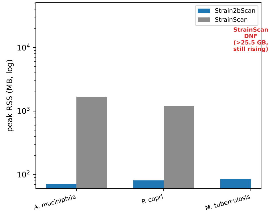
Peak memory
