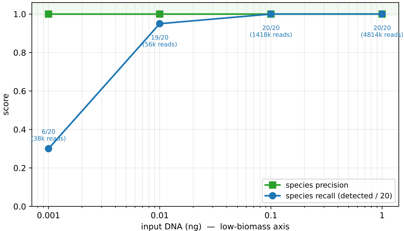
Real ATCC MSA-1002 mock (native Bcgl 2bRAD): precision 1.0 throughout, full recall down to 0.1 ng
