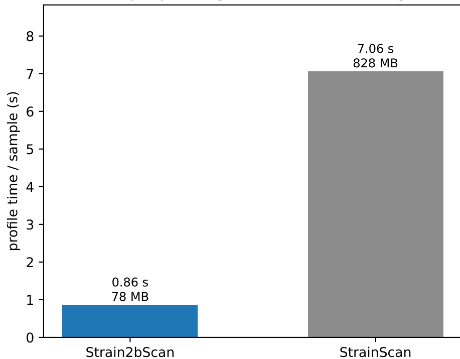
Per-sample profiling: \sim 8\times faster, \sim 11\times lighter
