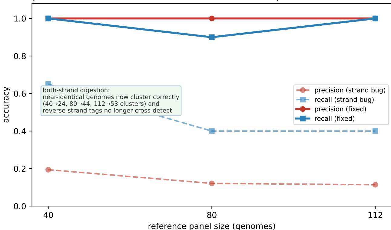
P. copri: a strand-invariance digestion fix, not a bigger panel (precision 0.19 \rightarrow 1.0; the 'recombination false uniqueness' was an artifact)
