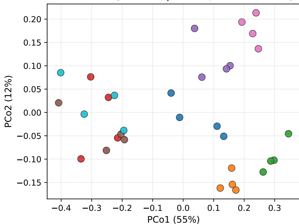
Strain-level ( R^2=0.83 , p=0.000 , 1-NN acc=91%)
