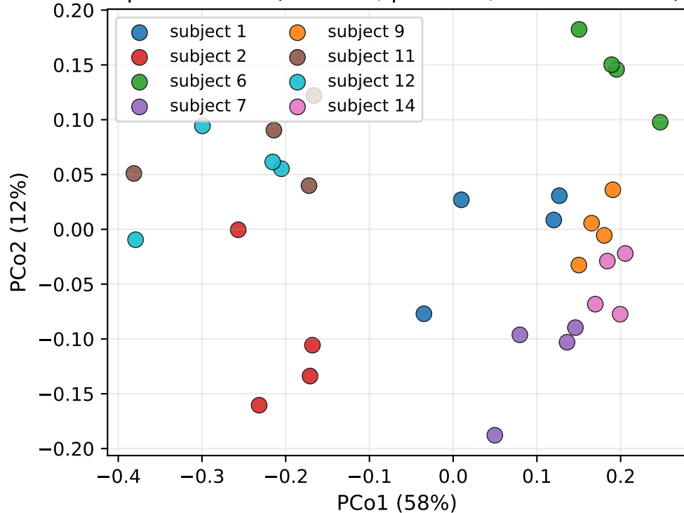
Species-level ( R^2=0.82 , p=0.000 , 1-NN acc=88%)
