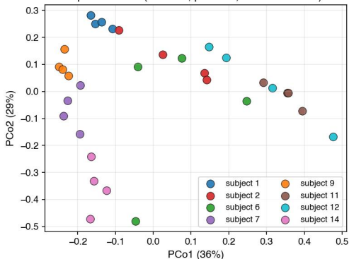
Species-level ( R^2=0.76 , p=0.000 , 1-NN acc=78%)
