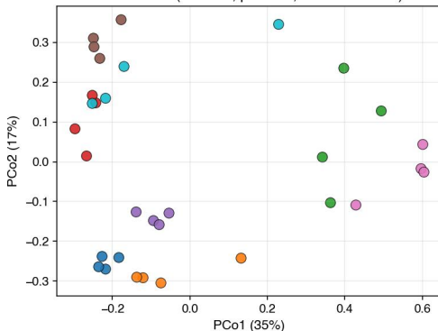
Strain-level ( R^2=0.76 , p=0.000 , 1-NN acc=97%)
