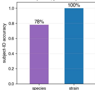
Leave-one-timepoint-out host-ID accuracy (train 3, predict 4th)
