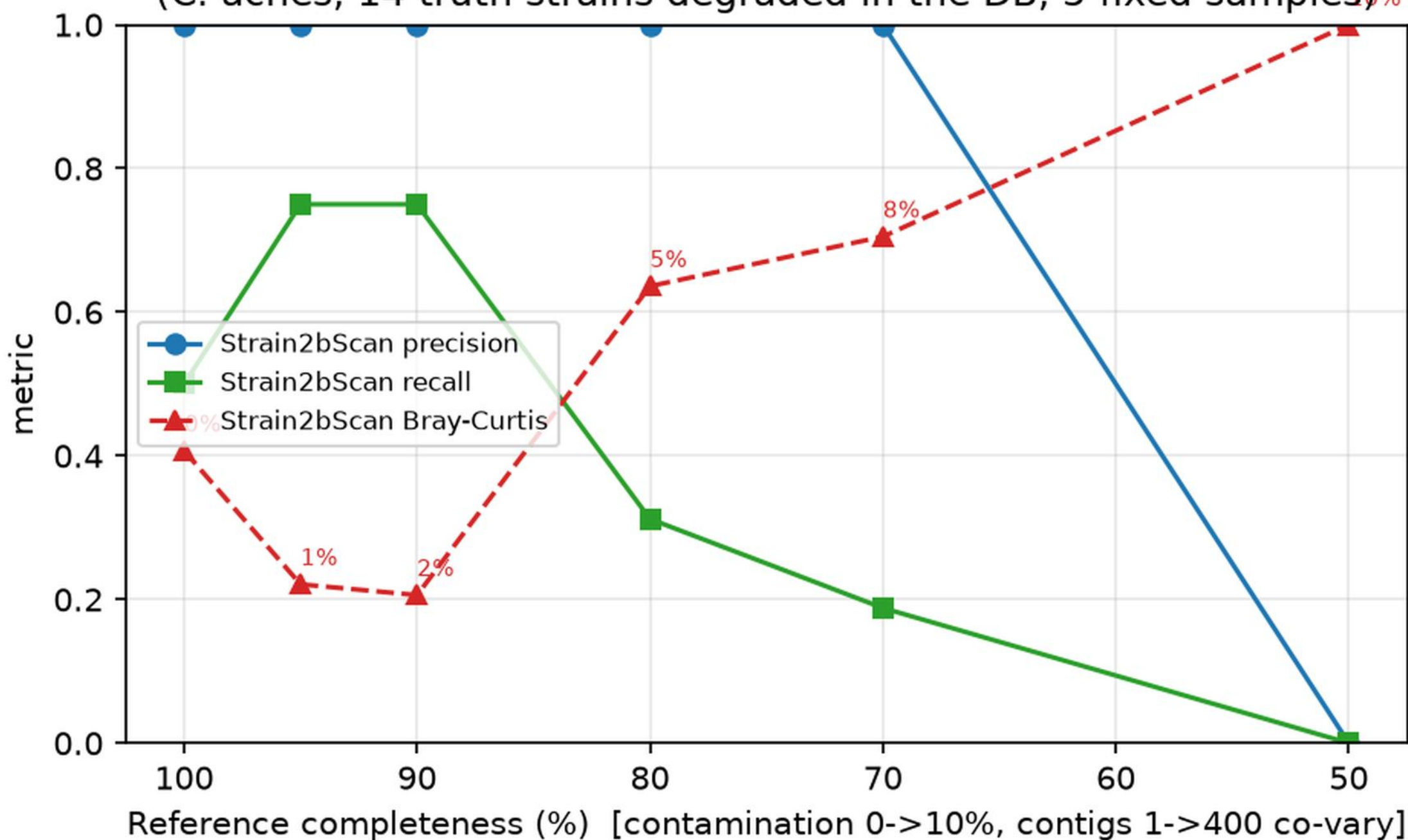
Reference-genome quality vs strain-profiling accuracy ( C. acnes , 14 truth strains degraded in the DB, 5 fixed samples)
