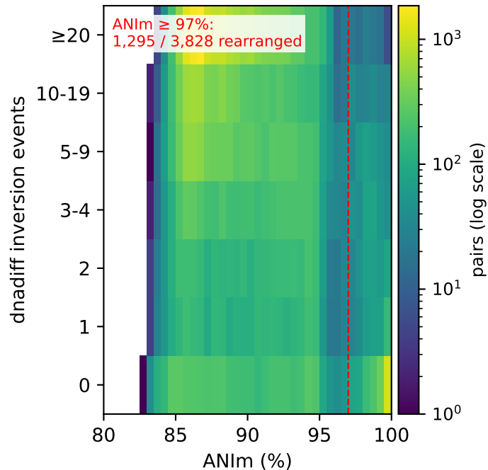
(a) Genome-wide ANI-rearrangement map
