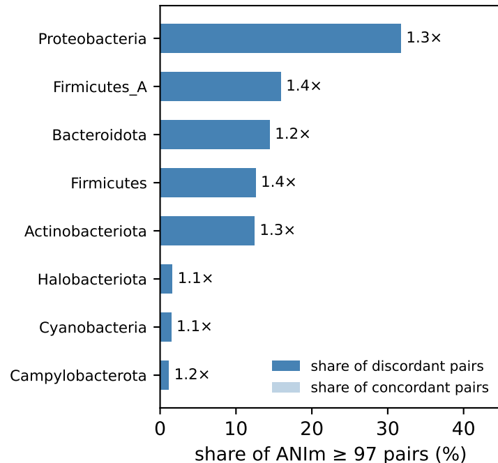
(c) Phylum enrichment
