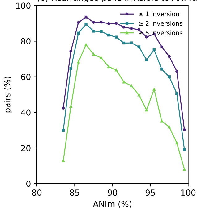
(b) Rearranged pairs invisible to ANI ranking
