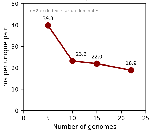
b Amortized pairwise cost
