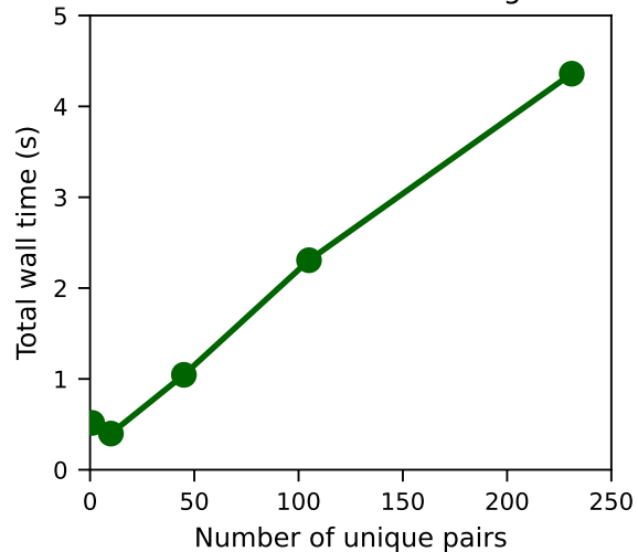
c Total runtime scaling
