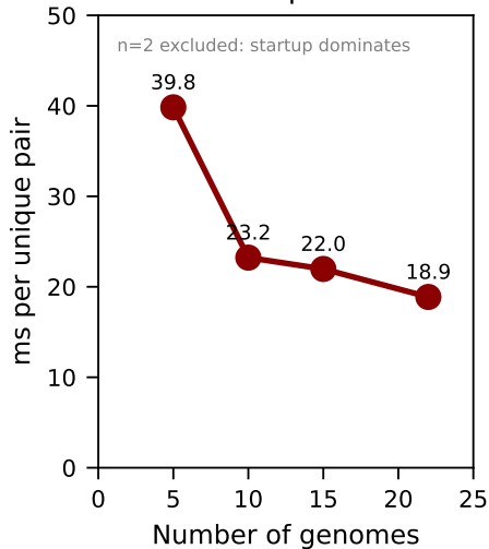
b Amortized pairwise cost
