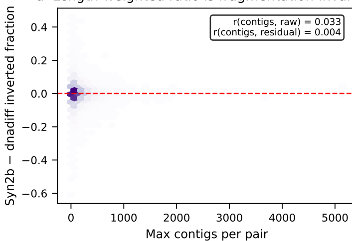
d Length-weighted ratio is fragmentation-invariant
