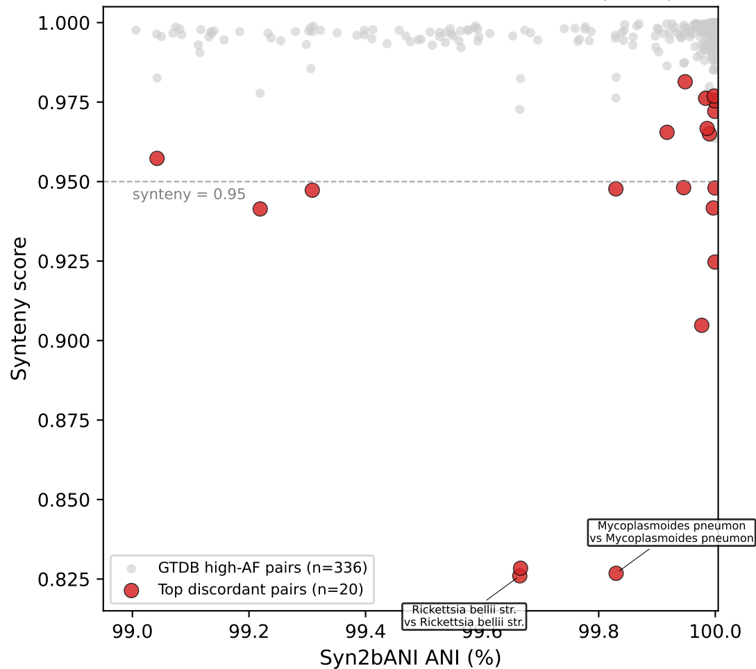
(a) Near-clonal ANI can coexist with low synteny
