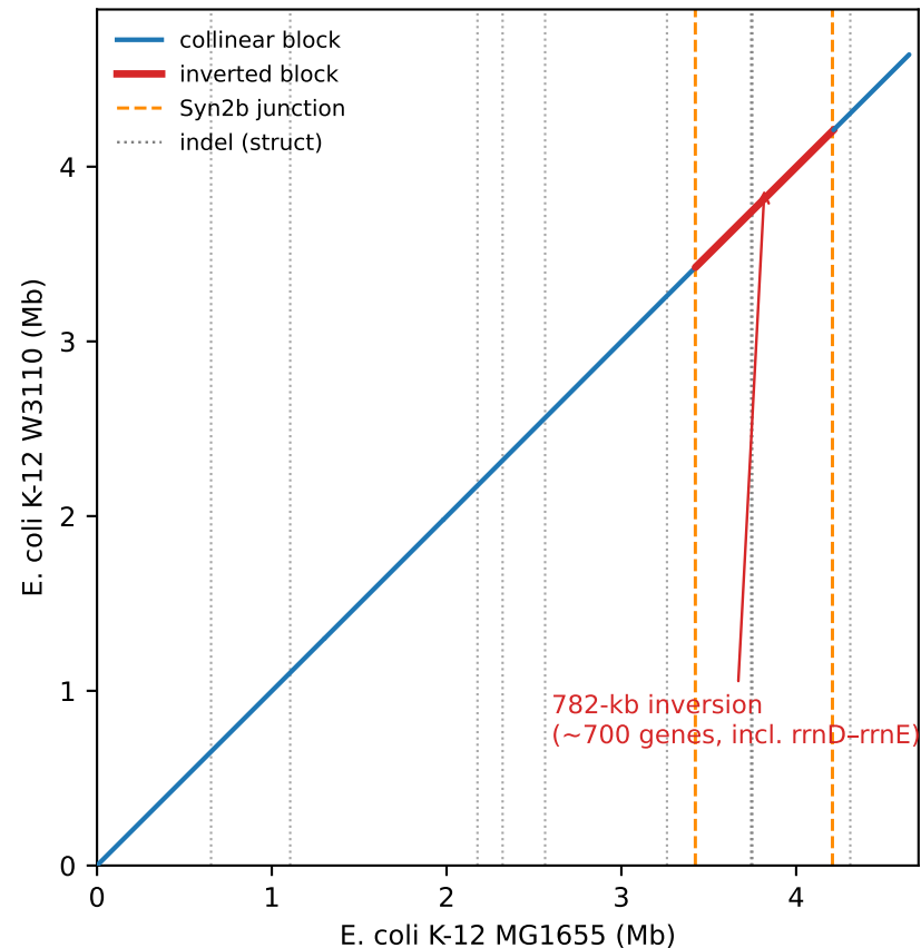
(a) Whole-genome alignment, MG1655 × W3110
