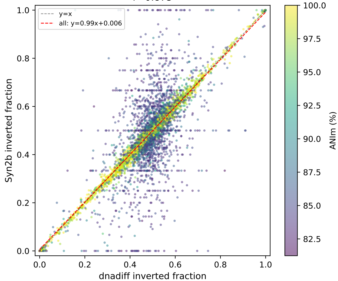
Extended high-ANI GTDB pairs (fixed-reference) (n=8937)
