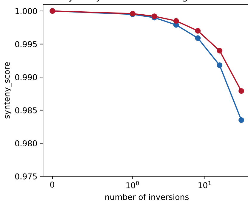
b synteny score vs rearrangement load
