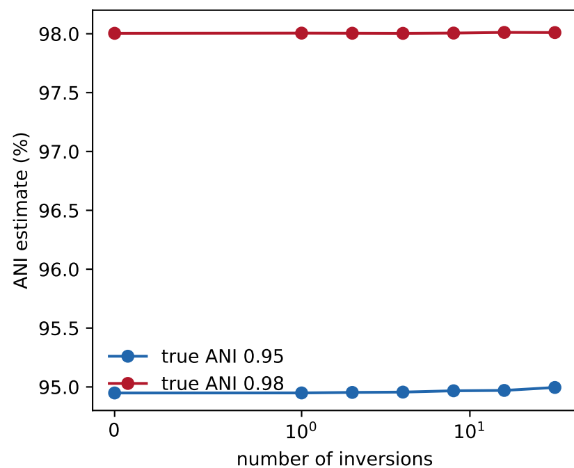
c ANI estimate is SV-invariant
