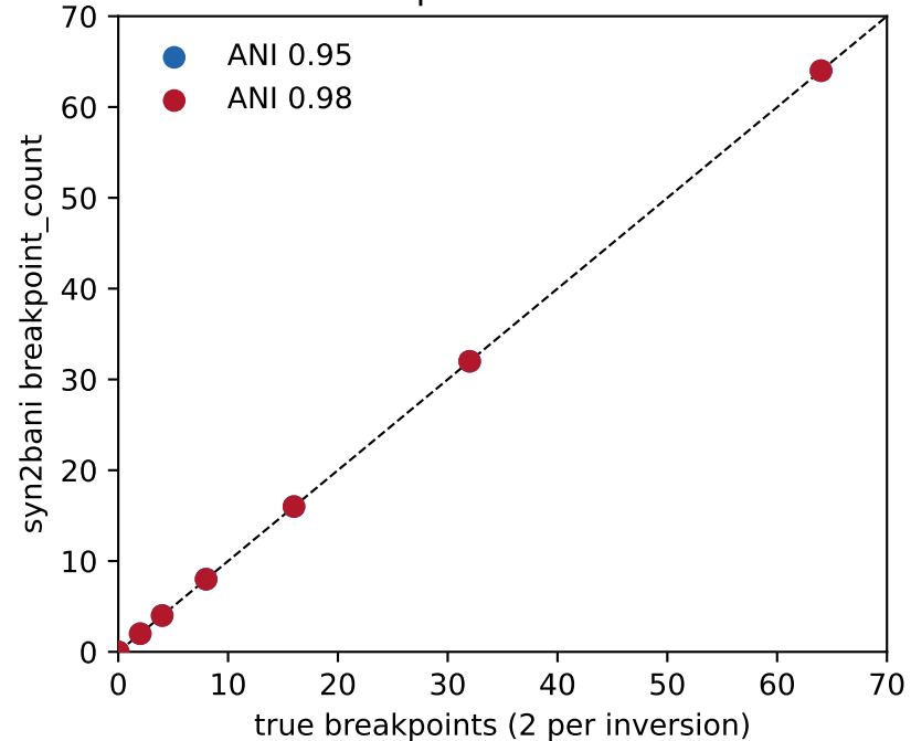
a breakpoint recall: exact
