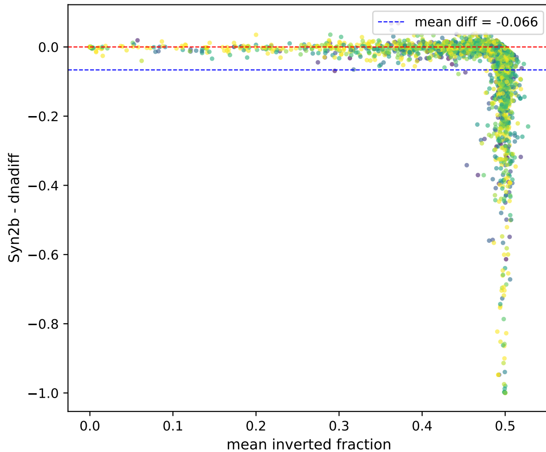
Bland-Altman
