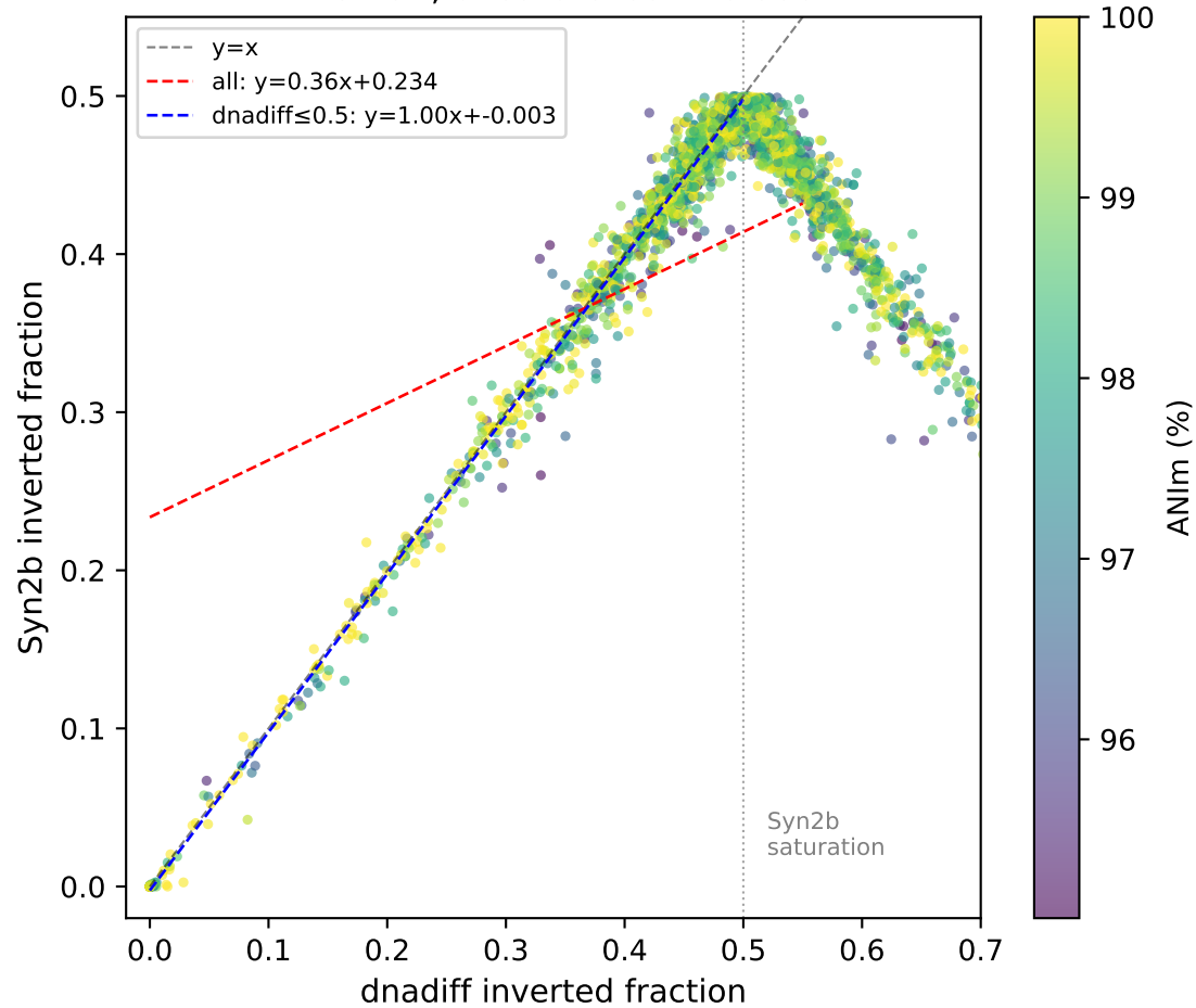
High-ANI GTDB pairs (n=2376) r=0.451 ; unsaturated r=0.995
