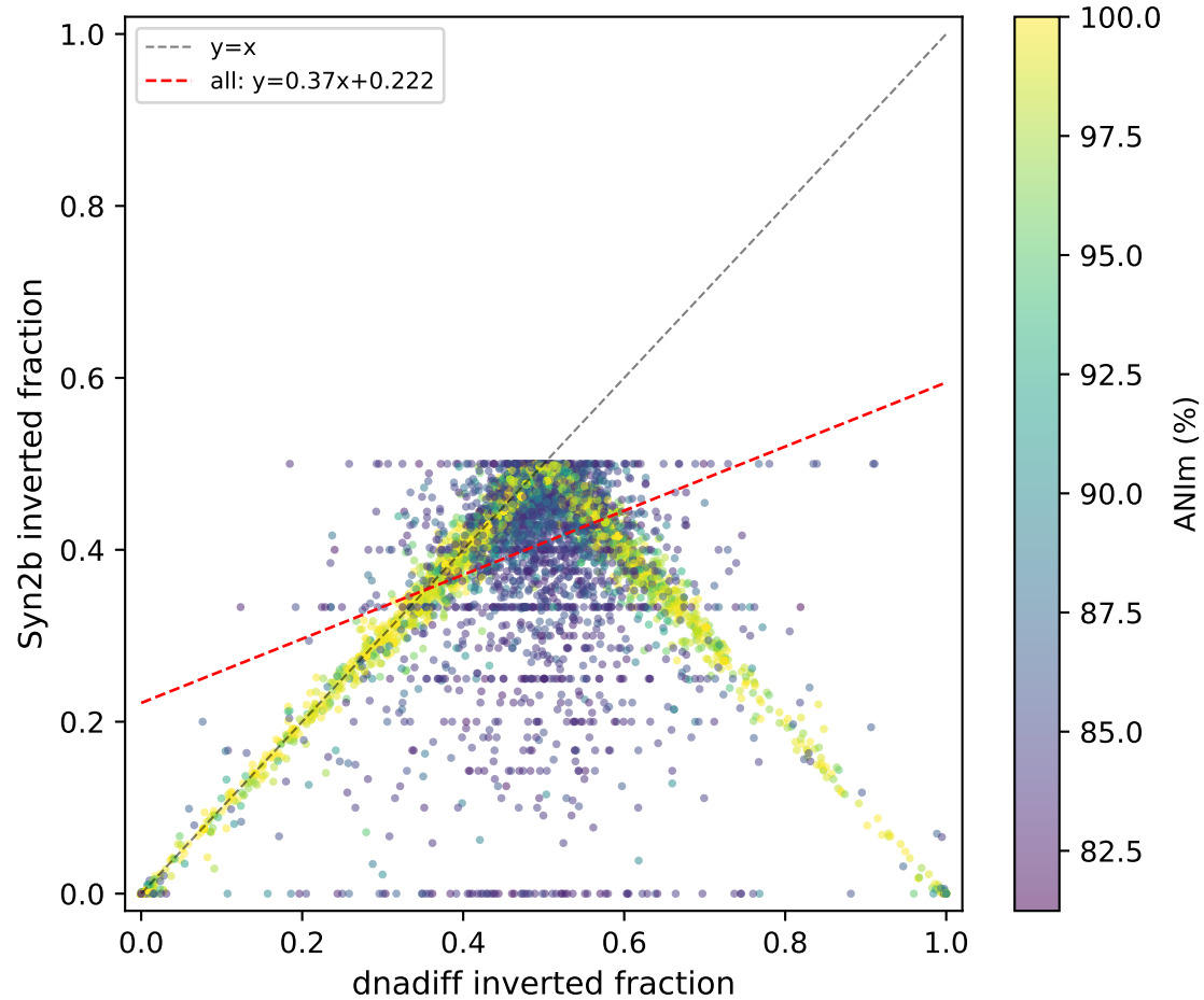
Extended high-ANI GTDB pairs (majority-frame) (n=8937)
