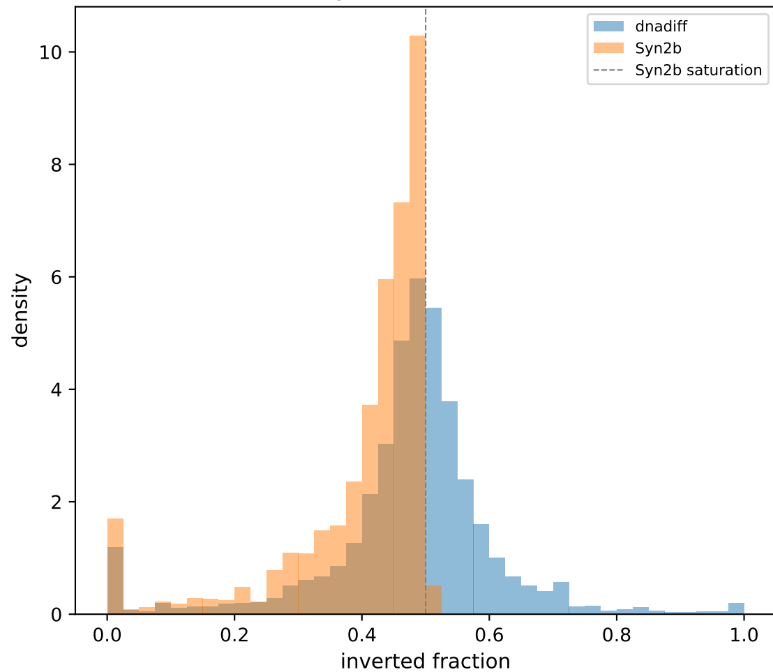
High-ANI distribution
