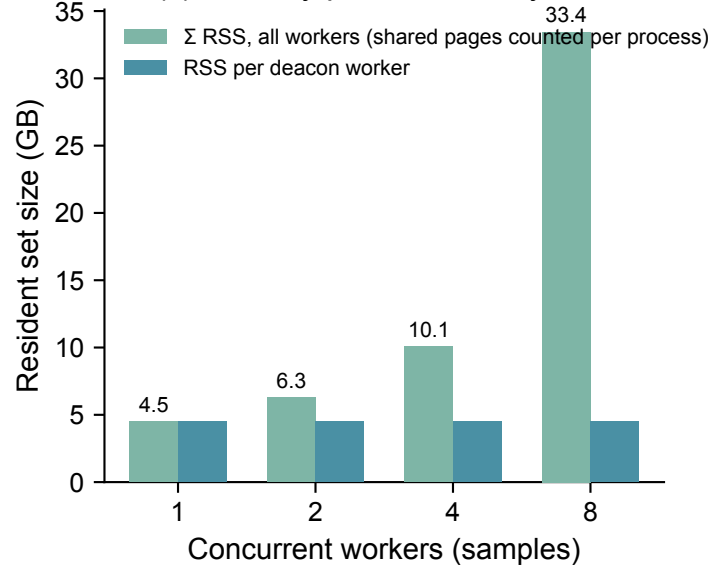
(c) Memory per worker stays flat
