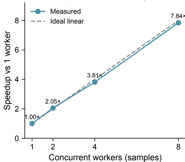
(b) Parallel efficiency
