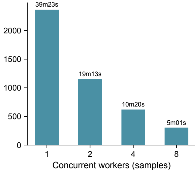
(a) Throughput scaling
