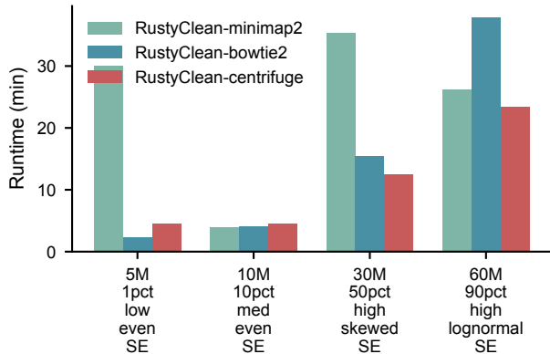
(a) Runtime
