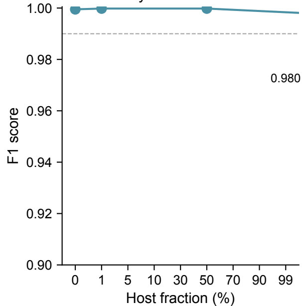
a Accuracy across host fractions
