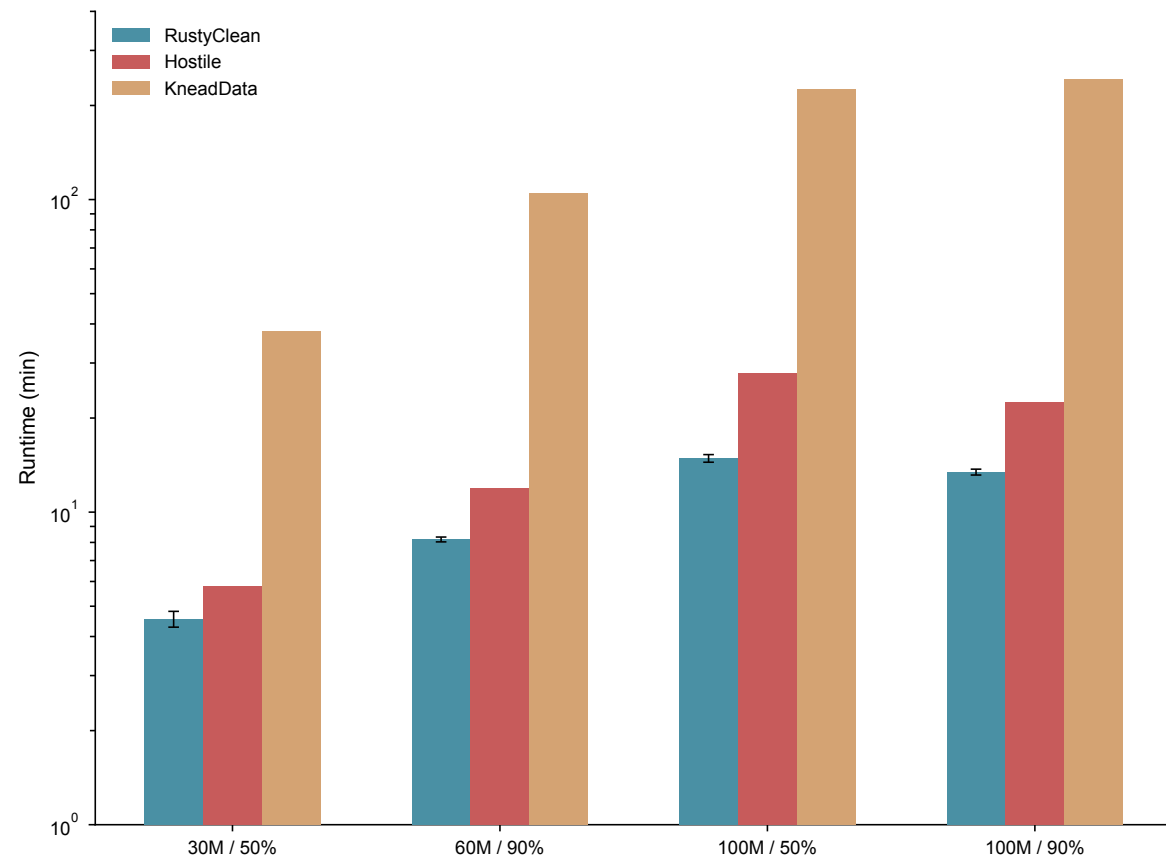
a Host-depletion runtime
