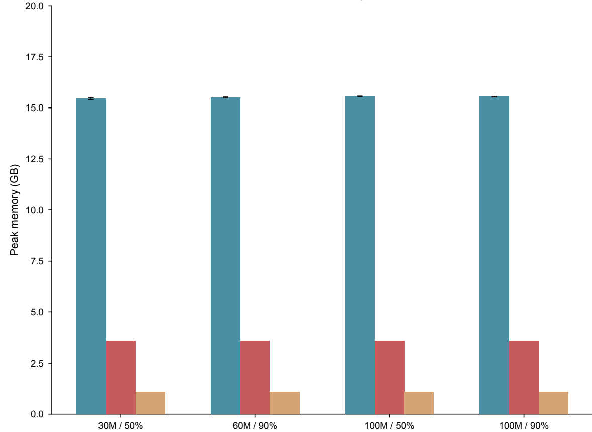
b Peak memory
