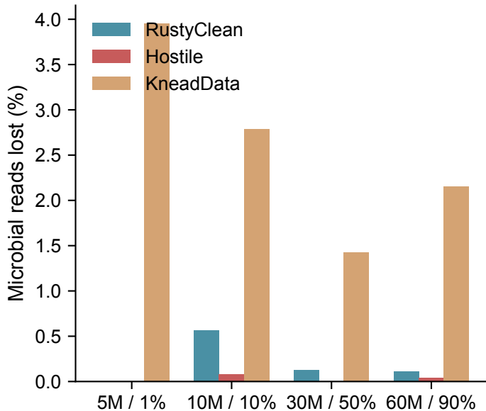
a Microbial read loss (false positives)
