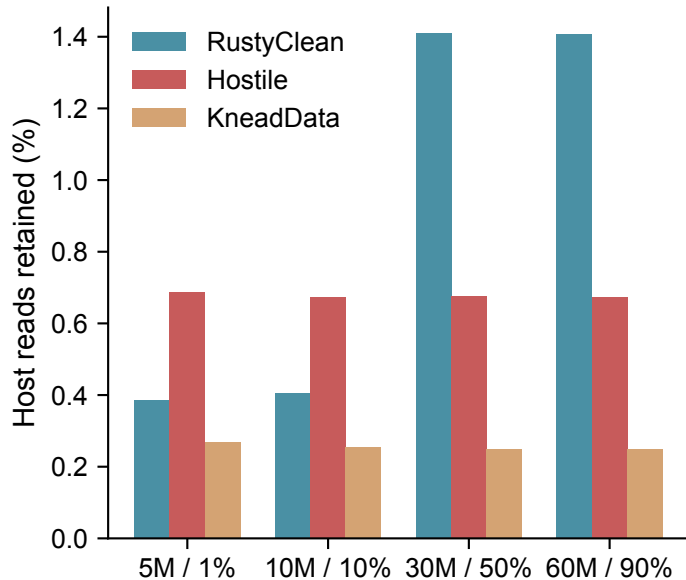
b Host carry-over (false negatives)
