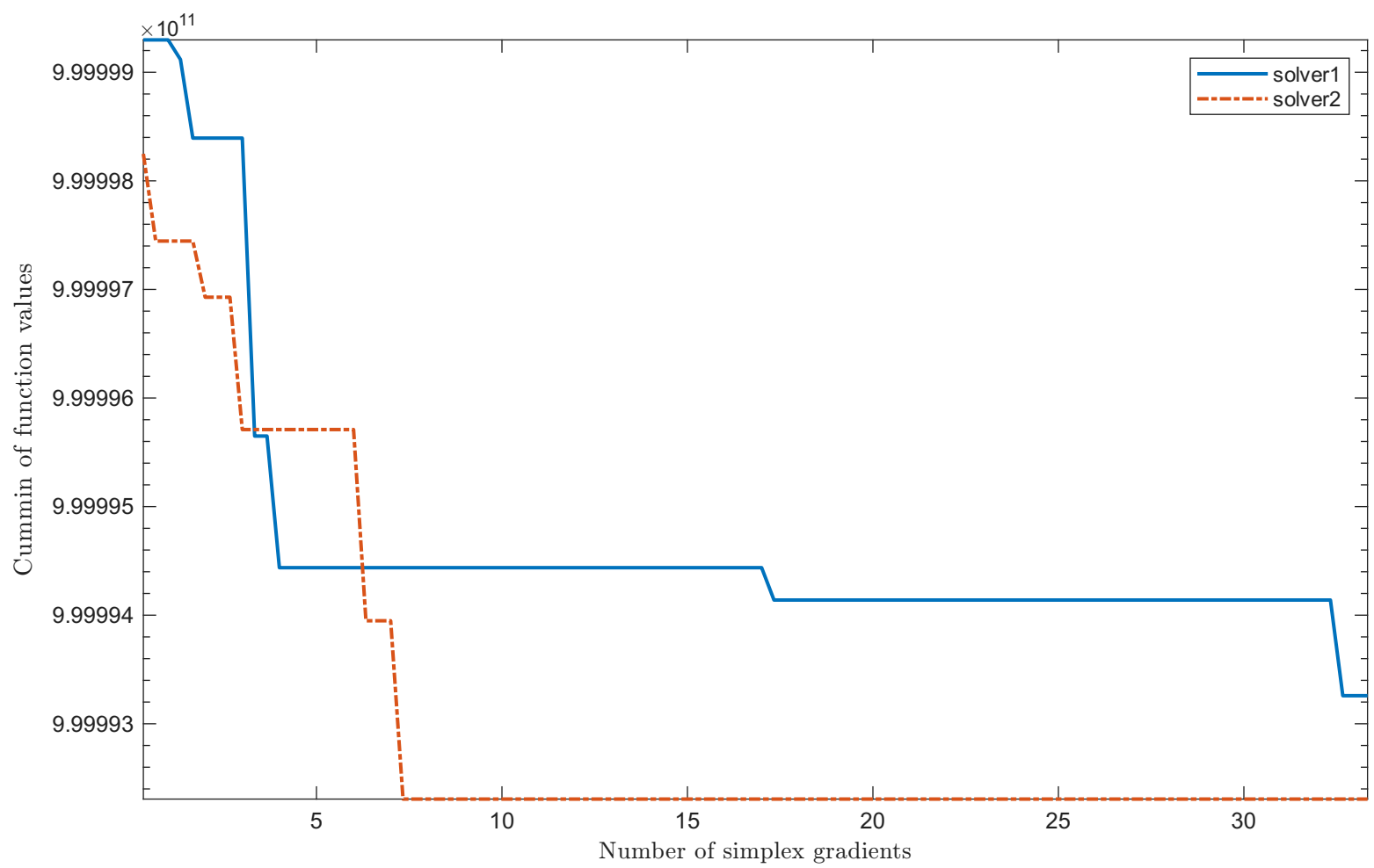
Cummin history profiles
