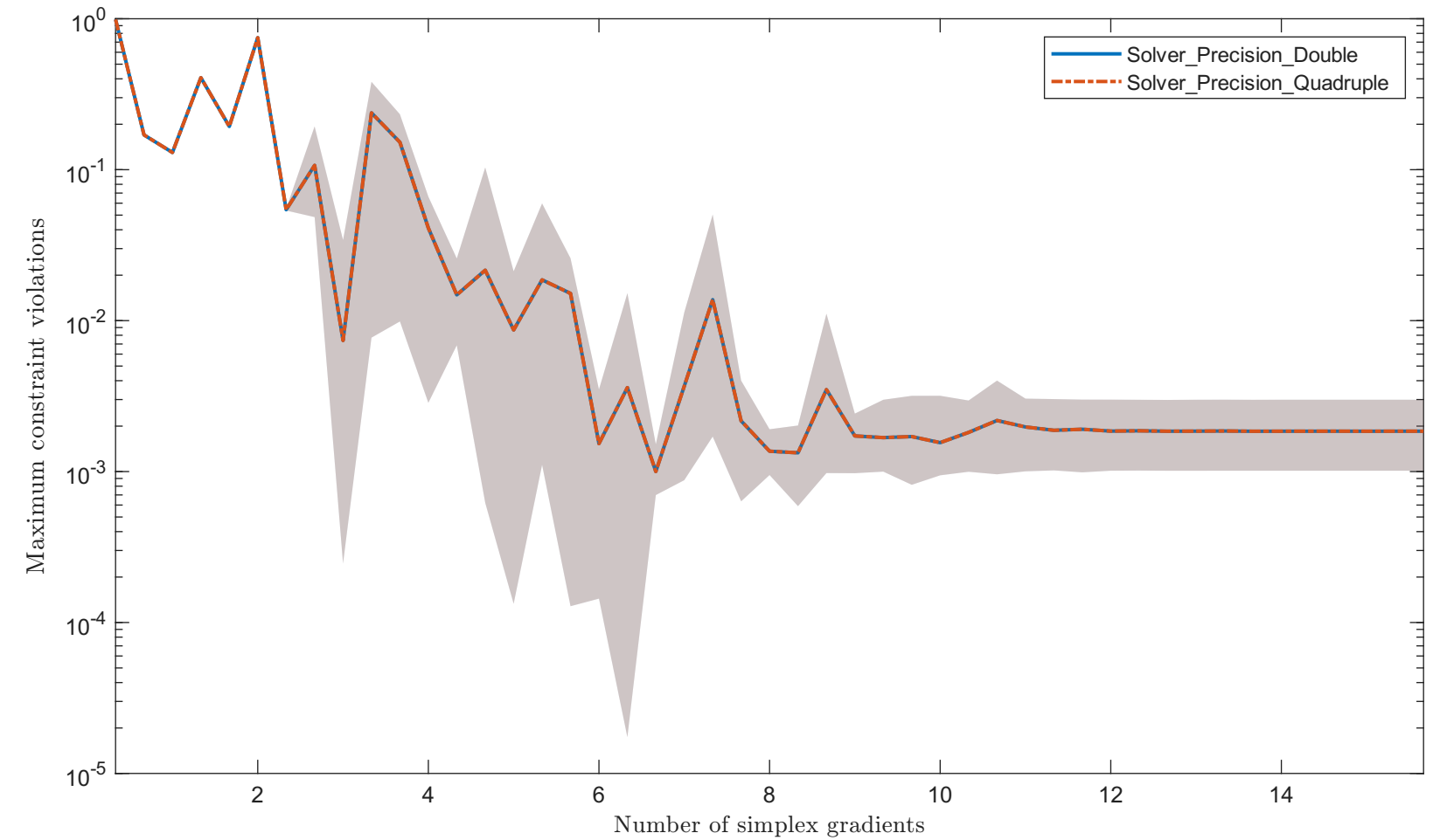
Solving "BT1" with "noisy_0.001_mixed_gaussian" feature
