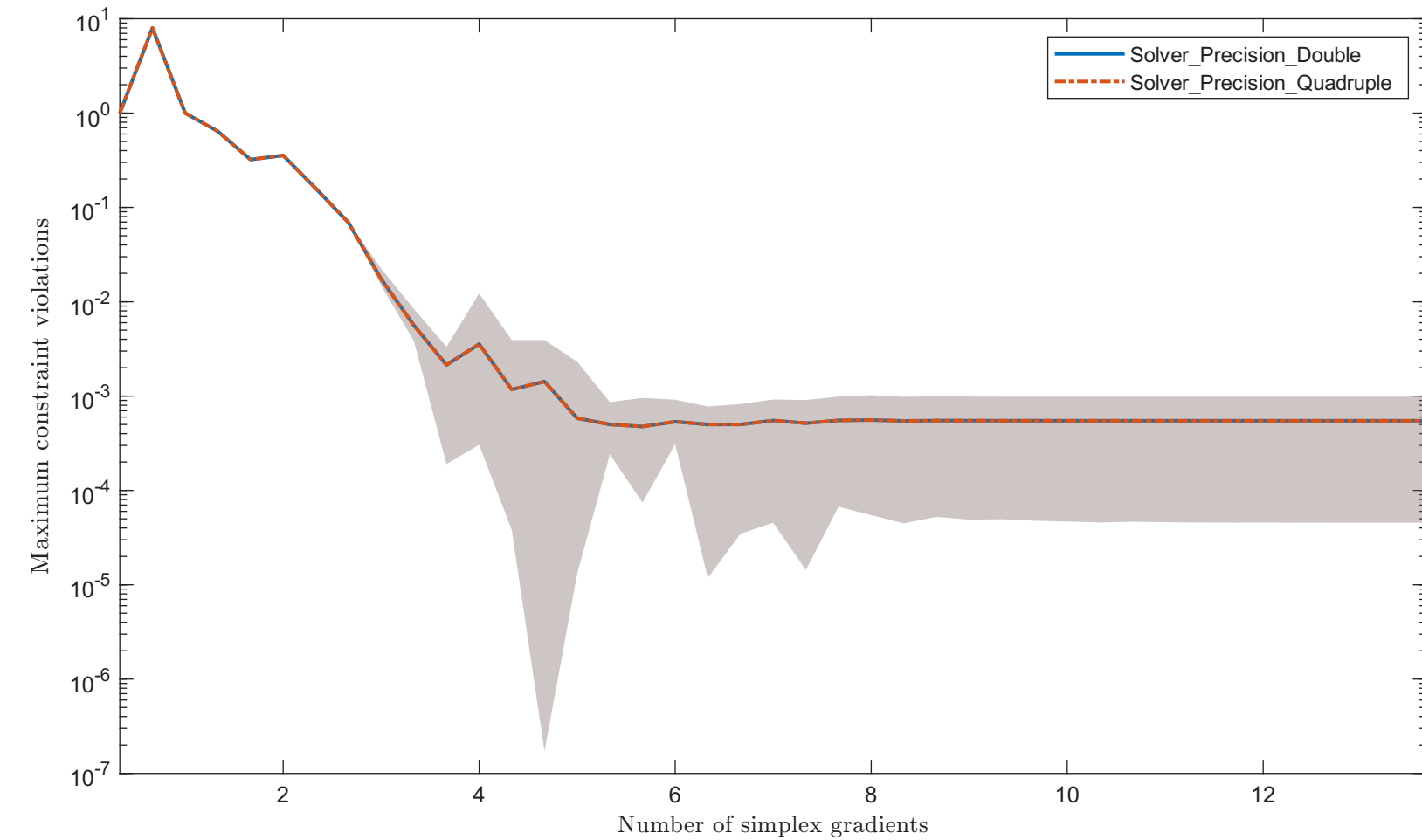
Solving "FLT" with "noisy_0.001_mixed_gaussian" feature
